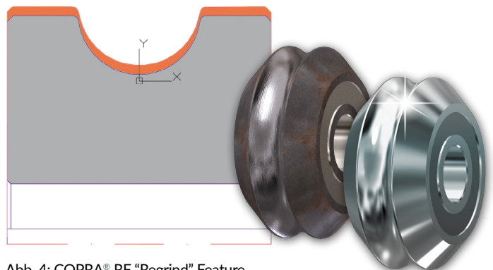
Abb. 4: COPRA® RF "Regrind" Feature
